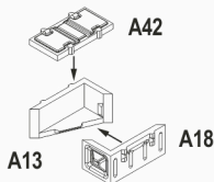
Steel Munition Box B167 Mk I
