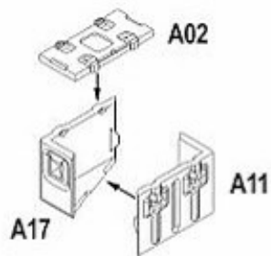
Steel Munition Box B166 Mk III
