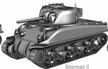
Sherman II Direct vision port, 75mm gun with M34 mantlet, low bustle turret, and T41 track links.
